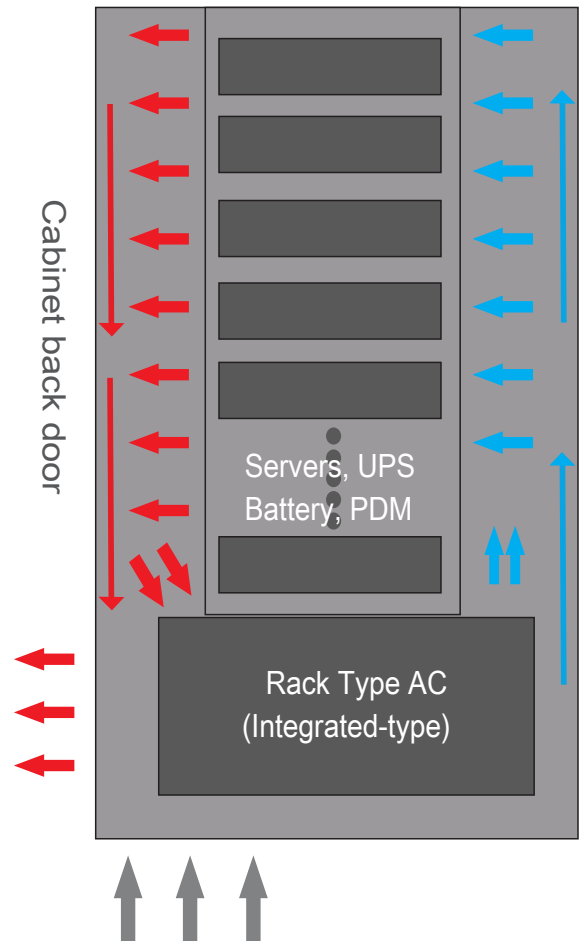
Scenario 2 Side view of single cabinet
